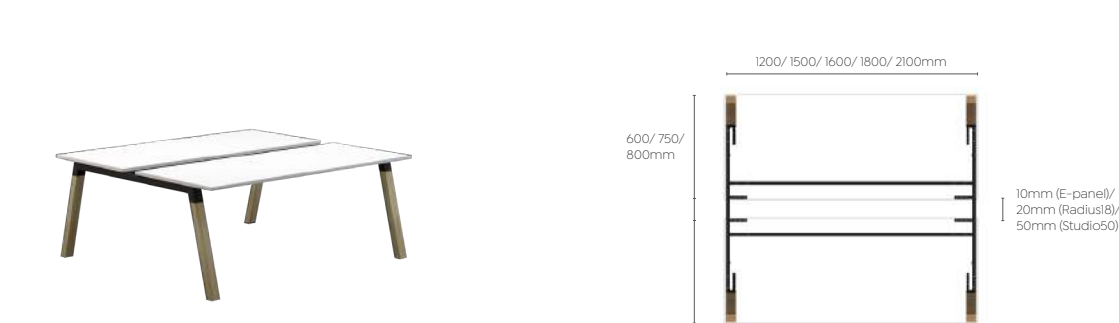
Plantation Double Sided Desks (Typical Frame Dimensions)
