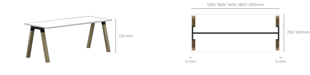
Plantation Single Desks (Typical Frame Dimensions)
