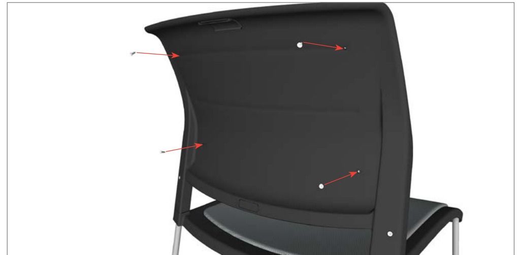
STEP 8: Pre-drill holes into the back shell, fully tighten the back pad to back shell with provided screws.
