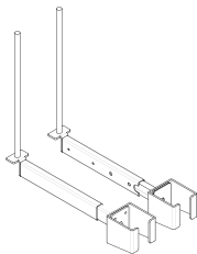
SSD Screen Brackets L/R Pair
